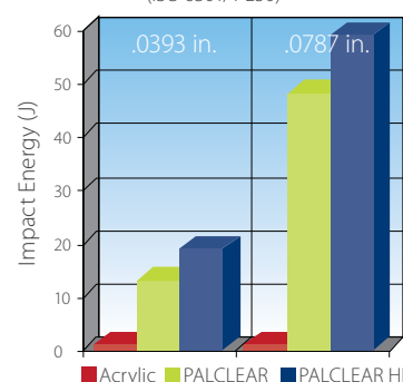
Impact Strength Comparison at 73°F (ISO 6301/1 E50)
