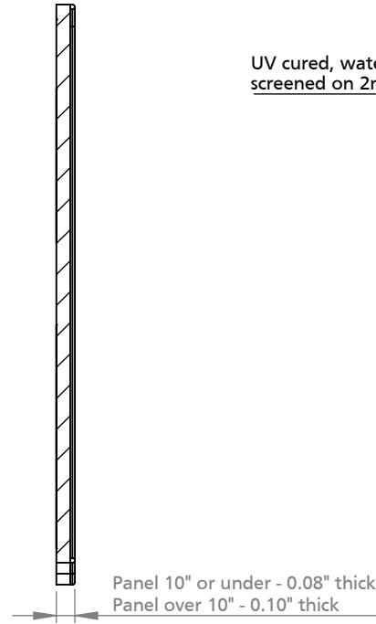
SECTION VIEW A-A II SCALE 1:1.5
