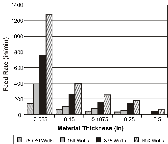
Typical Acrylic Cutting Speeds †
